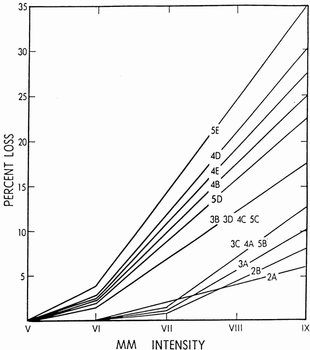
Motion-Damage Curve by Class of Construction for the San Francisco Bay Area. Descriptions of the Various Classes May Be Found in Table D.1. High-(H) and Low-(L) Rise Subclasses of Class 3 and Class 4 Have Been Combined.
