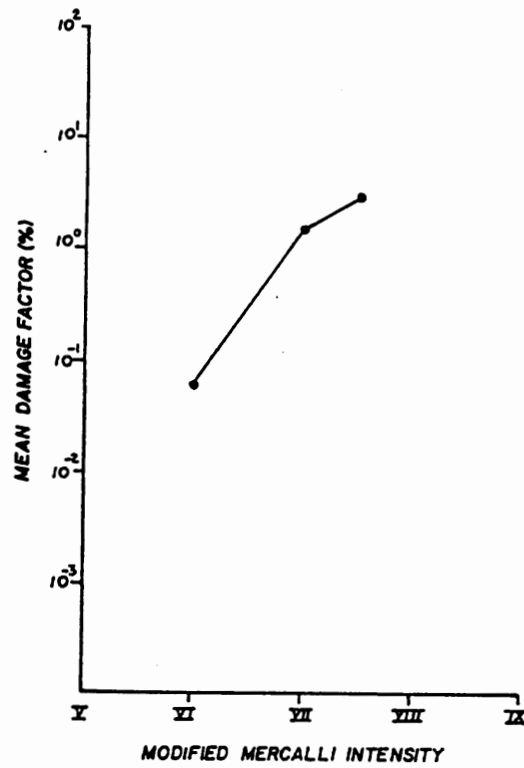
Damage versus Intensity Curve for All High-Rise Buildings During the 1971 San Fernando Earthquake. (Source: Whitman, Hong, and Reed, 1973)
