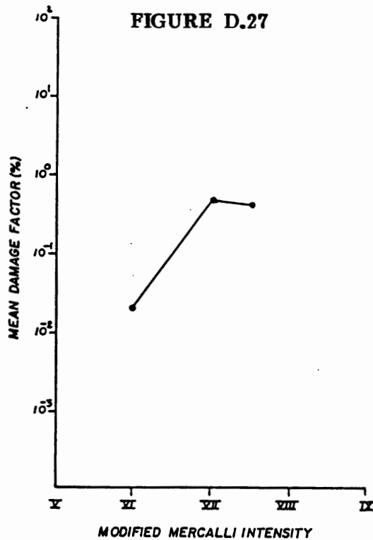
Damage versus Intensity Curve for Post-1947 Steel High-Rise Buildings During the 1971 San Fernando Earthquake. (Source: Whitman, Hong, and Reed, 1973)
