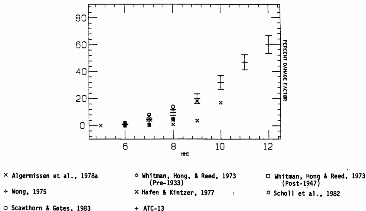
Motion-Damage Data from the Literature for High-Rise Reinforced Concrete Buildings. Also Shown are Mean and One Standard Deviation Bars for ATC-13 Damage-Factor Estimates.
