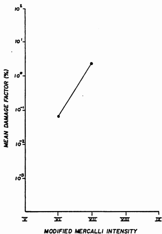
Damage versus Intensity Curves for Pre-1933 Steel High-Rise Buildings During the 1971 San Fernando Earthquake. (Source: Whitman, Hong, and Reed, 1973)
