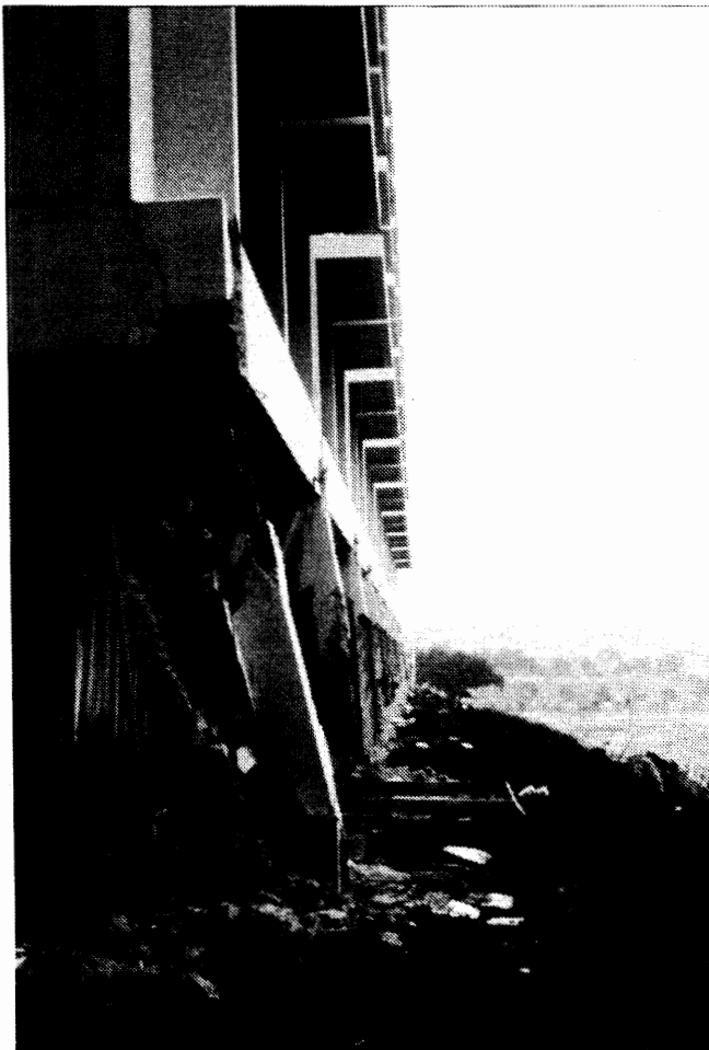
a. Overall View Showing Collapsed End Stairwells, but Generally Good Condition of Upper Portions of Building.
