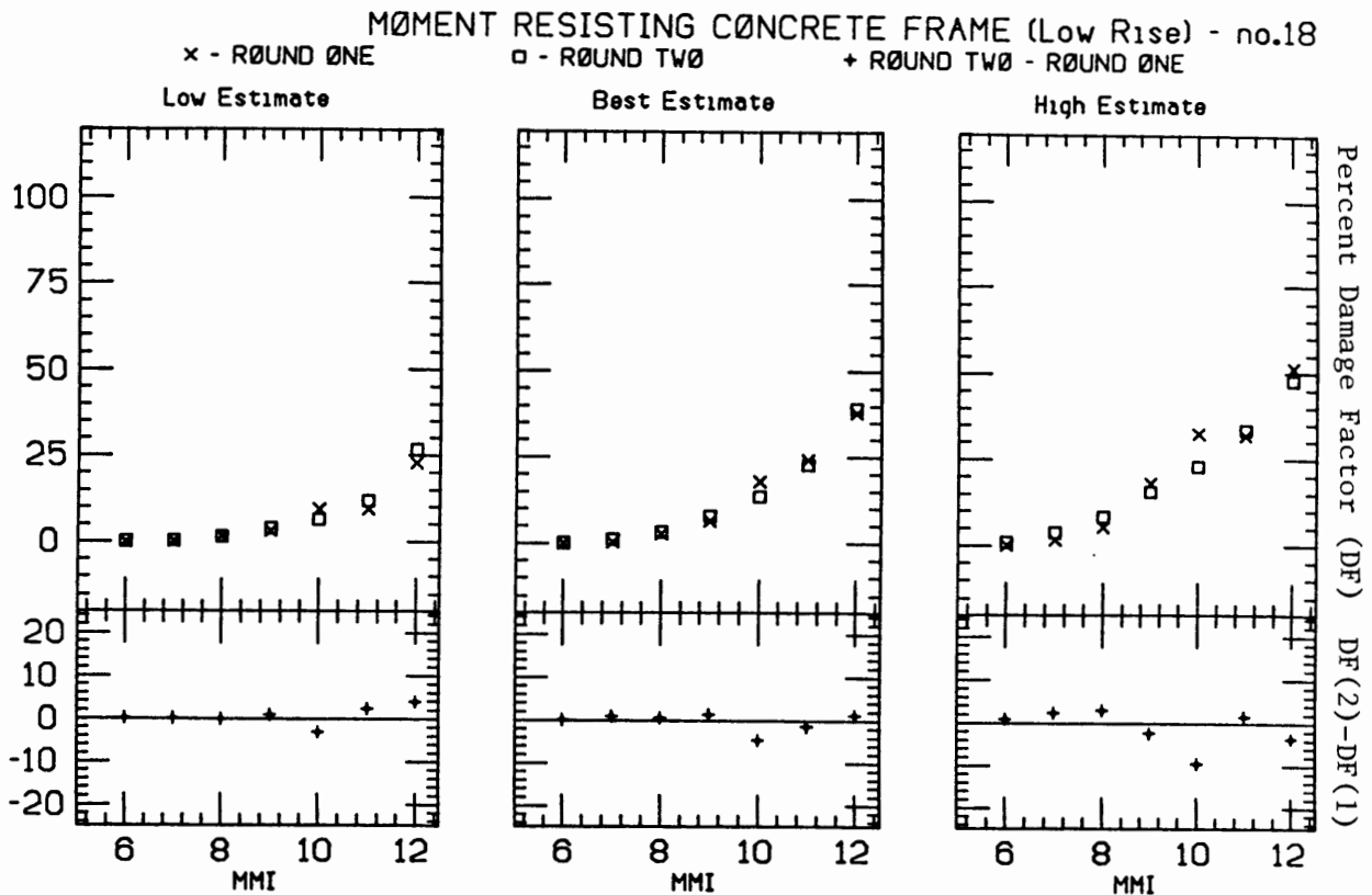
Comparison Between Round One and Two Mean Responses (Damage Factor Questionnaire).
