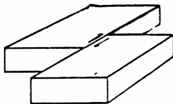
STRIKE-SLIP FAULT
