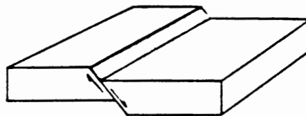
NORMAL-SLIP FAULT
