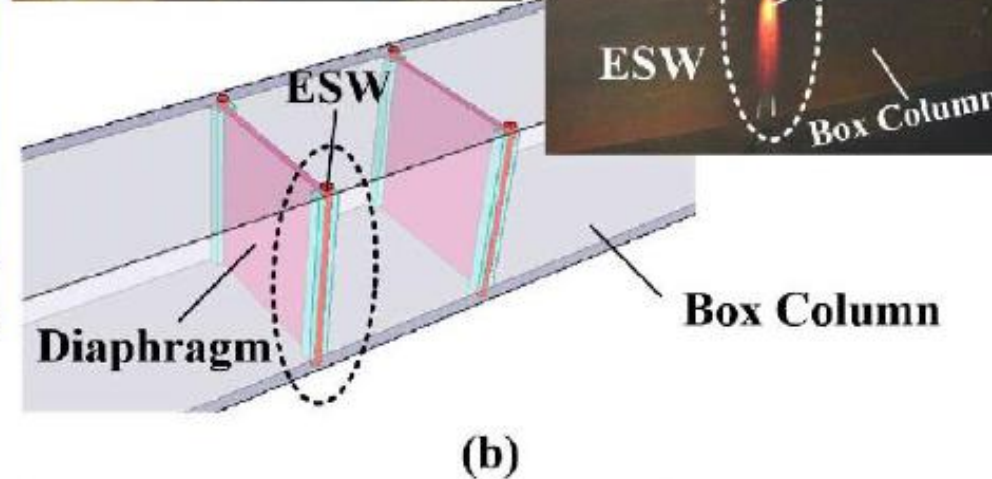
Figure 1. (a) Schematics of the steel beam-to-box column connection and (b) the electro-slag
