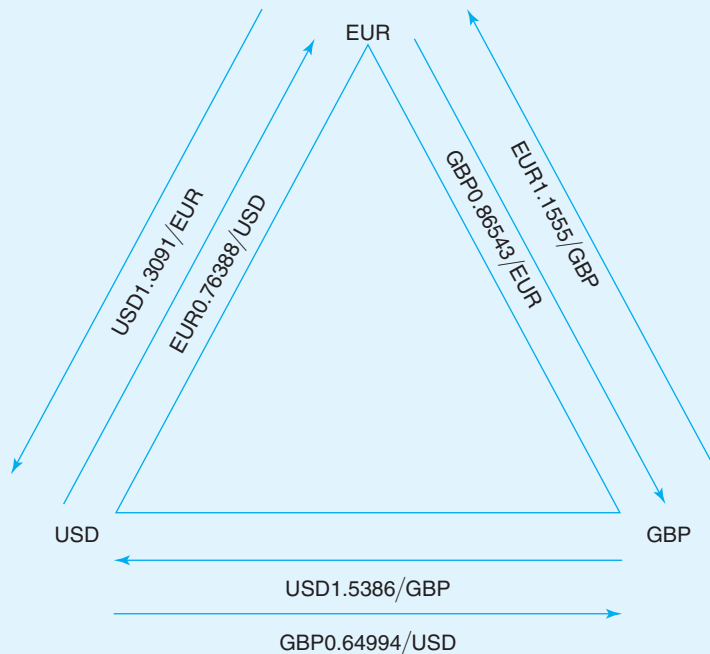
Exhibit 2.7 Triangular Arbitrage Diagram
