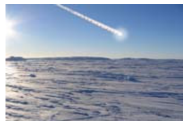
شدت (Intensity)
